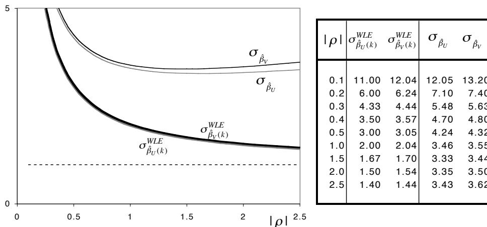
Figure 2: “Rulers” of the asymptotic standard deviations of \hat{\beta}_U(k; \rho) , \hat{\beta}_V(k; \rho) , WLE_{\hat{\beta}_U(k; \rho), \rho} and WLE_{\hat{\beta}_V(k; \rho), \rho} , for \gamma = \beta = 1 .
